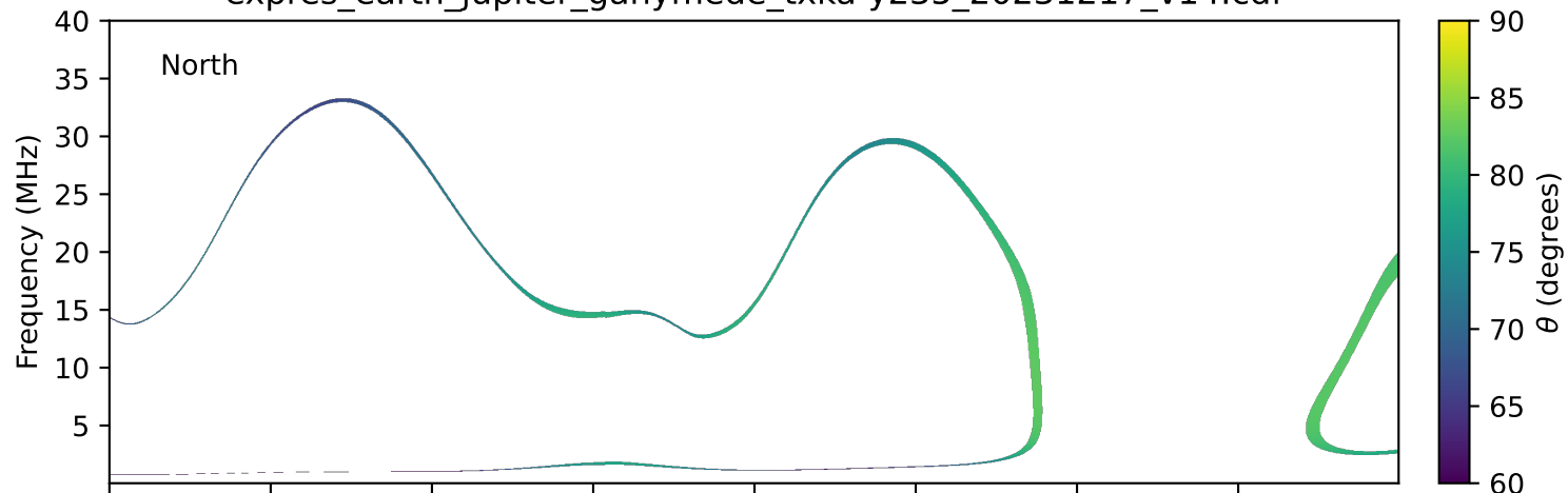
expres_earth_jupiter_ganymede_txka-y235_20231217_v14.cdf
