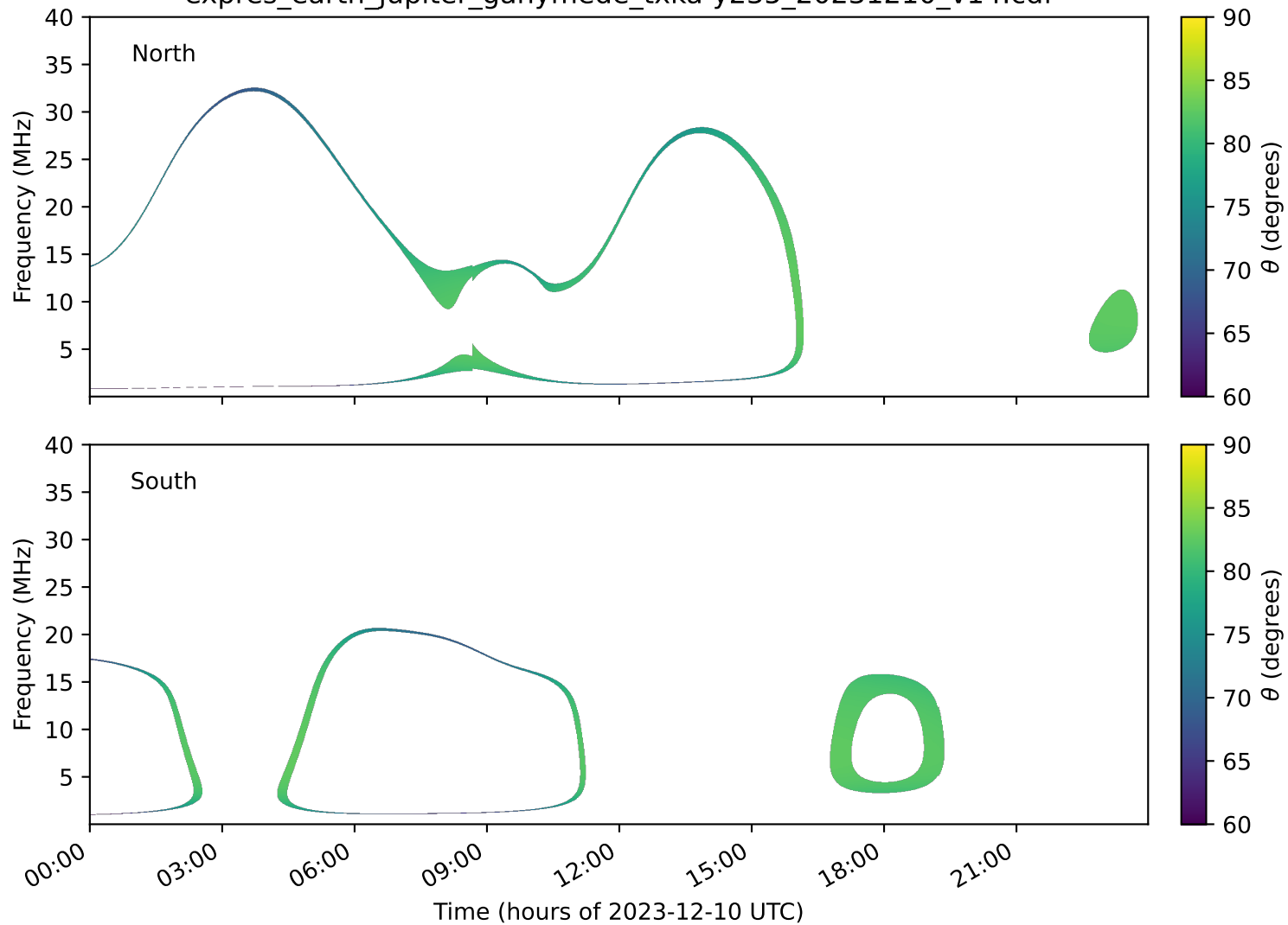
expres_earth_jupiter_ganymede_txka-y235_20231210_v14.cdf
