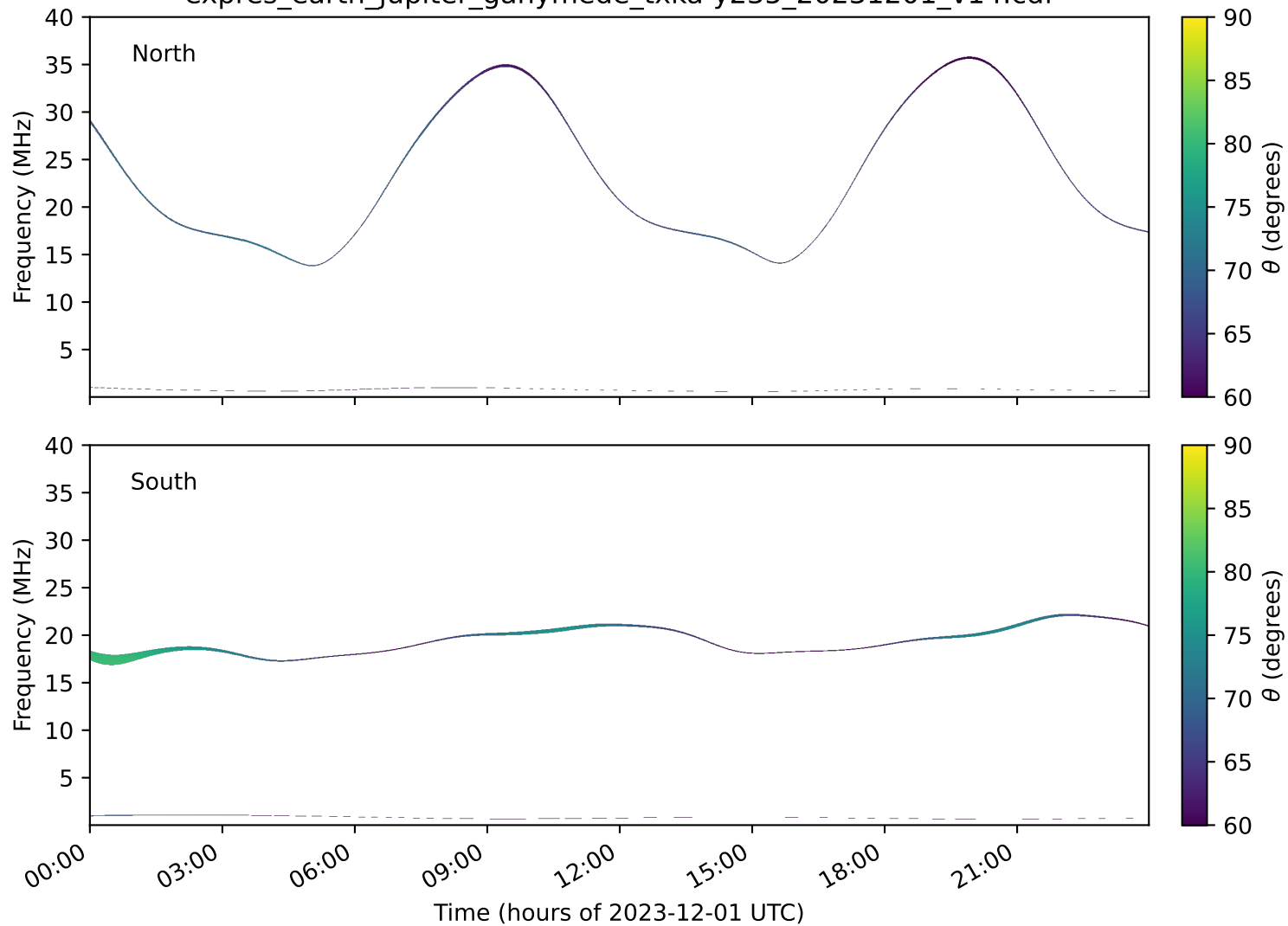
expres_earth_jupiter_ganymede_txka-y235_20231201_v14.cdf
