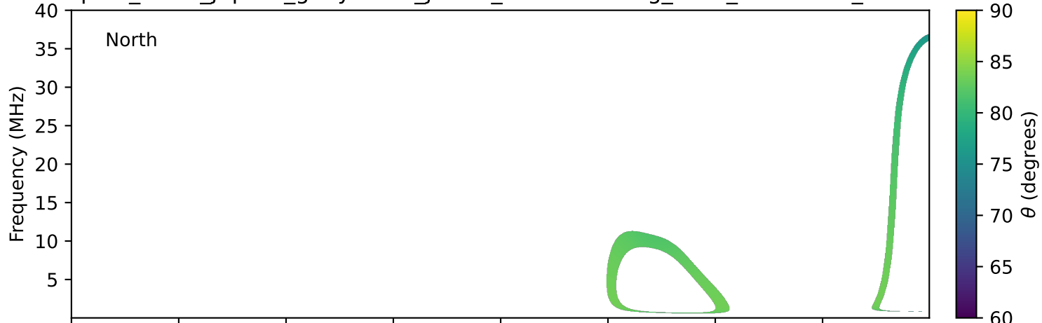
expres_earth_jupiter_ganymede_jrm33_lossc-wid1deg_3kev_20231214_v11.cdf
