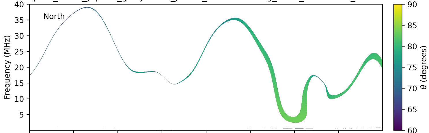
expres_earth_jupiter_ganymede_jrm33_lossc-wid1deg_3kev_20231210_v11.cdf
