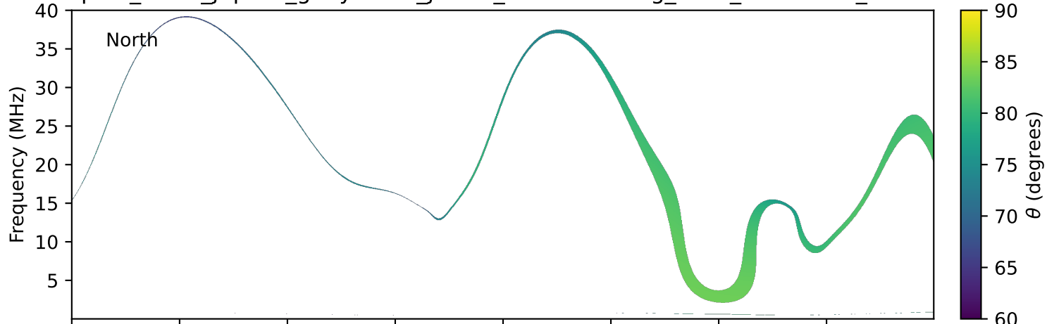
expres_earth_jupiter_ganymede_jrm09_lossc-wid1deg_3kev_20231210_v11.cdf
