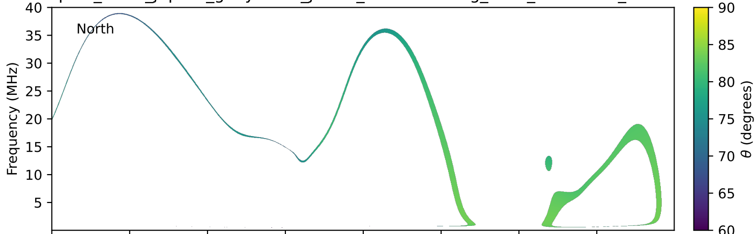
expres_earth_jupiter_ganymede_jrm09_lossc-wid1deg_3kev_20231203_v11.cdf
