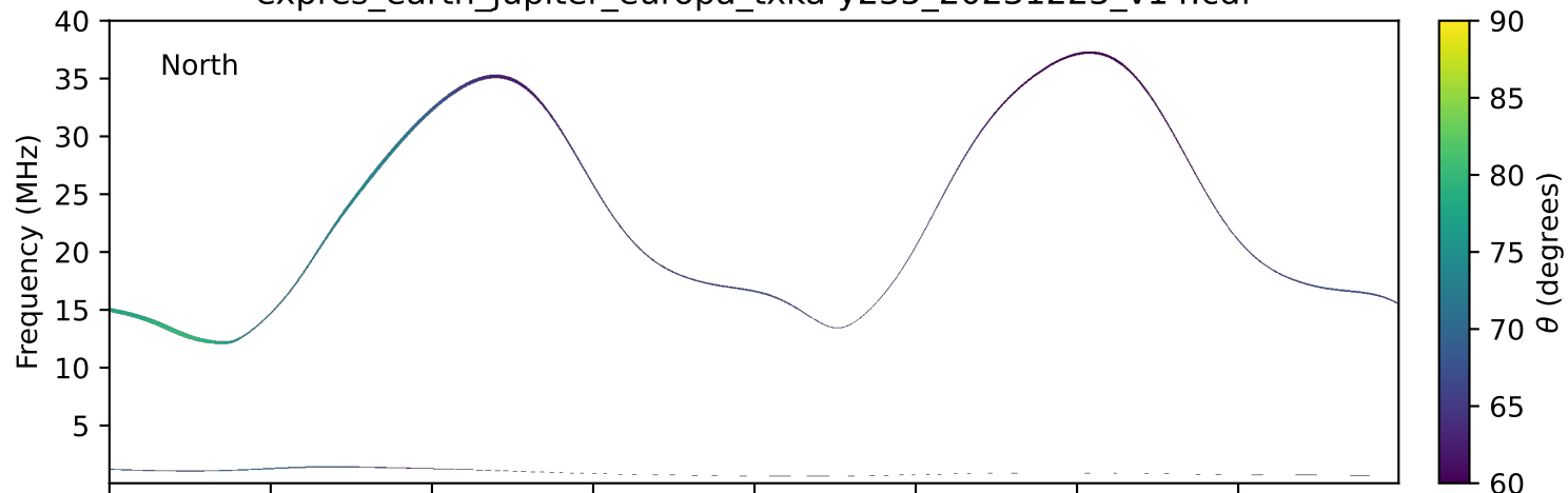
expres_earth_jupiter_europa_txka-y235_20231223_v14.cdf
