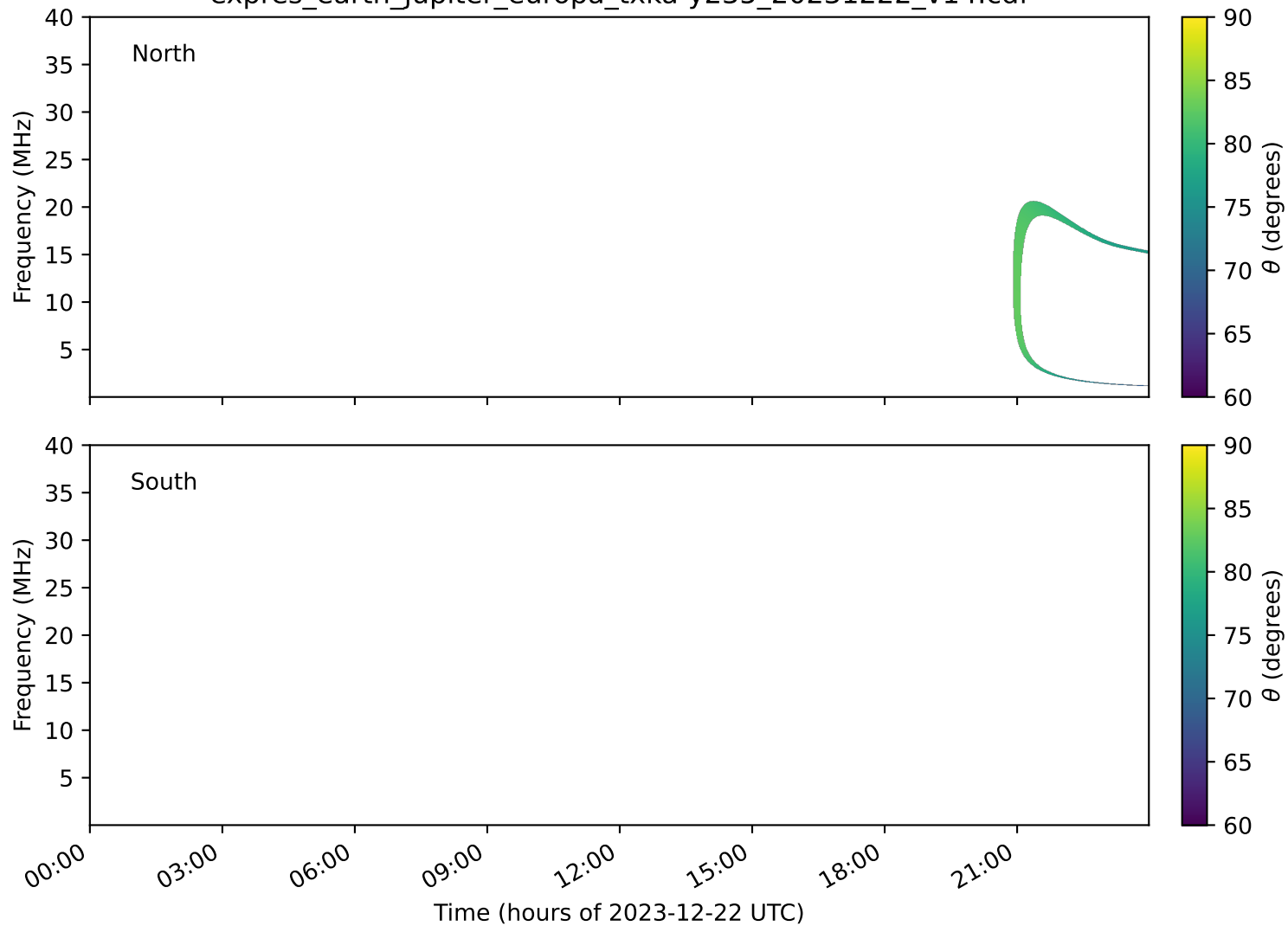
expres_earth_jupiter_europa_txka-y235_20231222_v14.cdf
