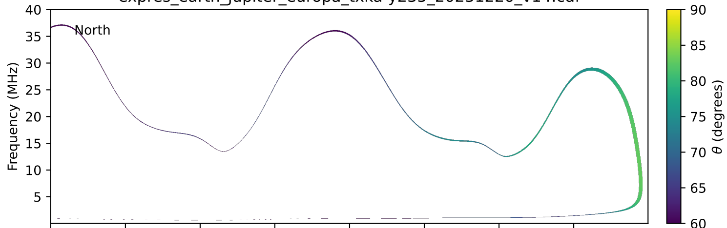
expres_earth_jupiter_europa_txka-y235_20231220_v14.cdf
