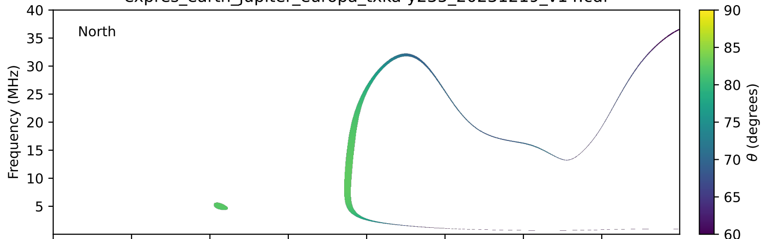
expres_earth_jupiter_europa_txka-y235_20231219_v14.cdf
