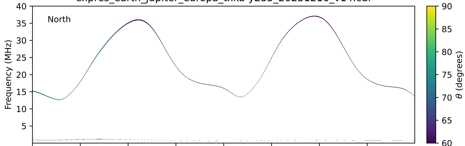
expres_earth_jupiter_europa_txka-y235_20231216_v14.cdf
