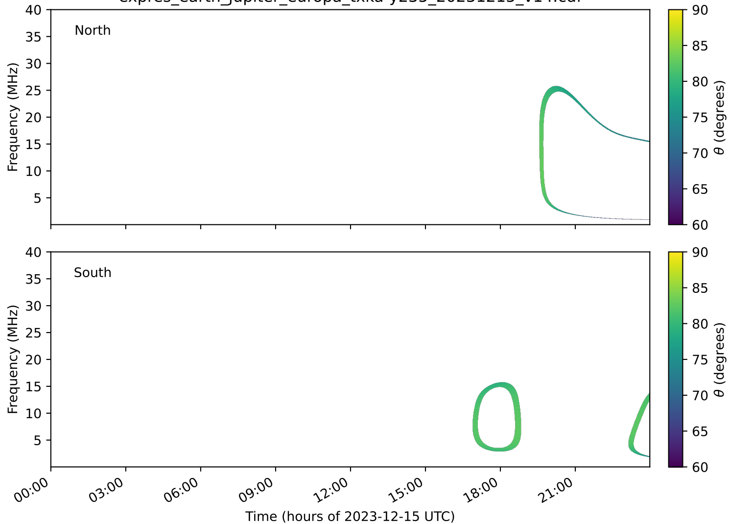
expres_earth_jupiter_europa_txka-y235_20231215_v14.cdf
