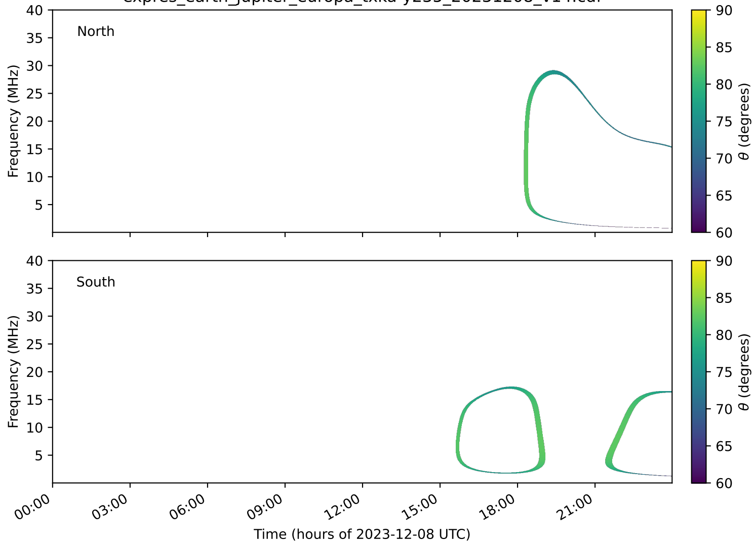
expres_earth_jupiter_europa_txka-y235_20231208_v14.cdf
