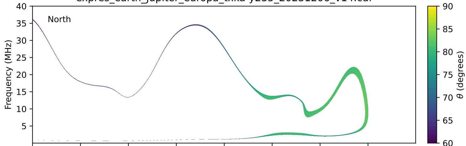
expres_earth_jupiter_europa_txka-y235_20231206_v14.cdf
