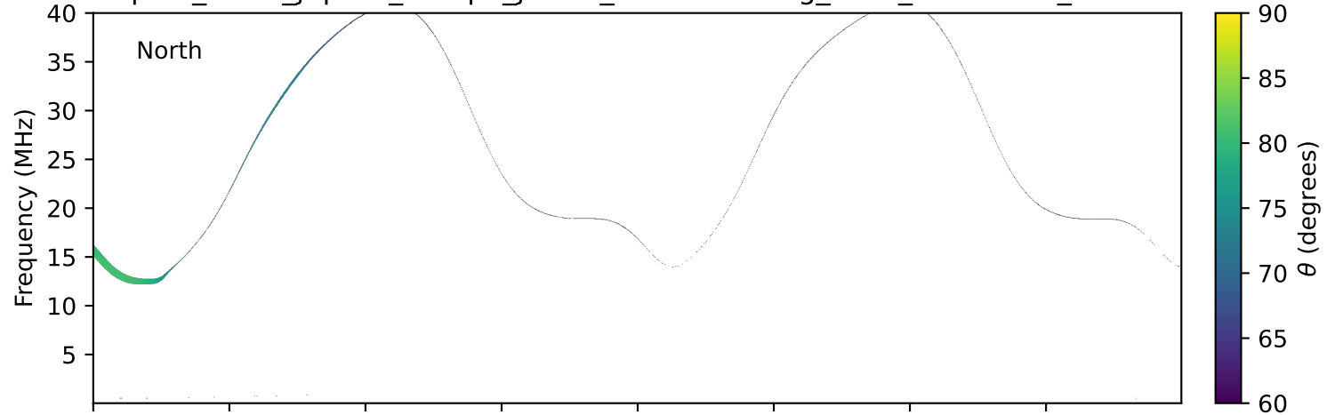
expres_earth_jupiter_europa_jrm33_lossc-wid1deg_3kev_20231216_v11.cdf
