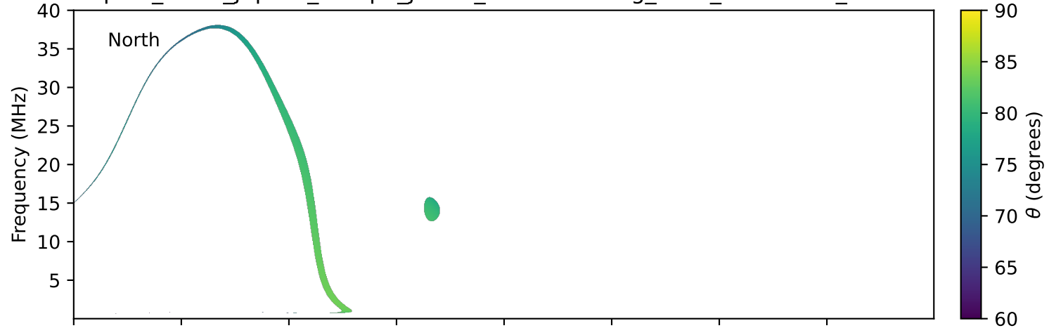
expres_earth_jupiter_europa_jrm33_lossc-wid1deg_3kev_20231210_v11.cdf
