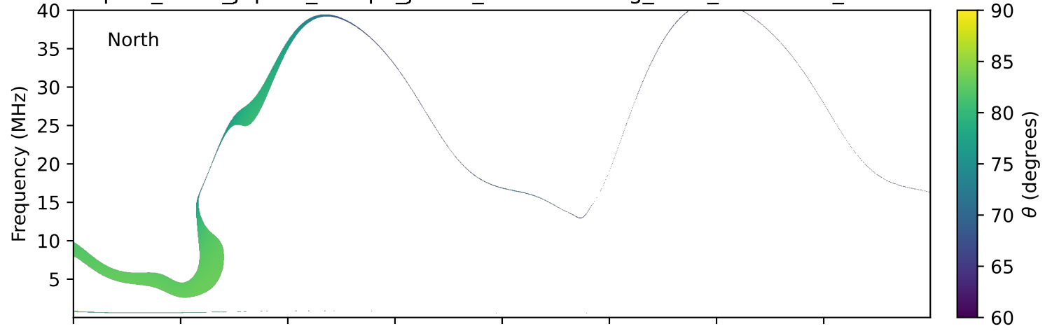
expres_earth_jupiter_europa_jrm09_lossc-wid1deg_3kev_20231230_v11.cdf
