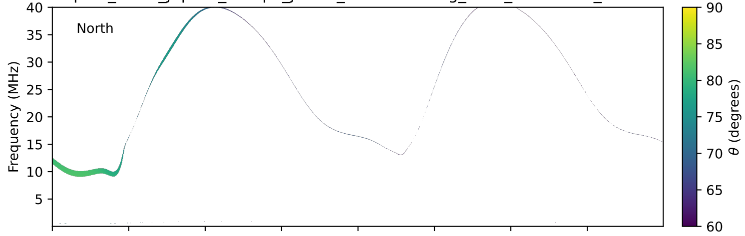
expres_earth_jupiter_europa_jrm09_lossc-wid1deg_3kev_20231223_v11.cdf
