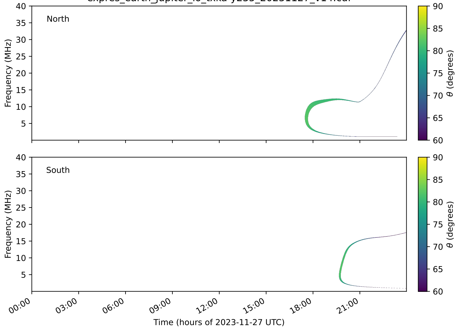
expres_earth_jupiter_io_txka-y235_20231127_v14.cdf
