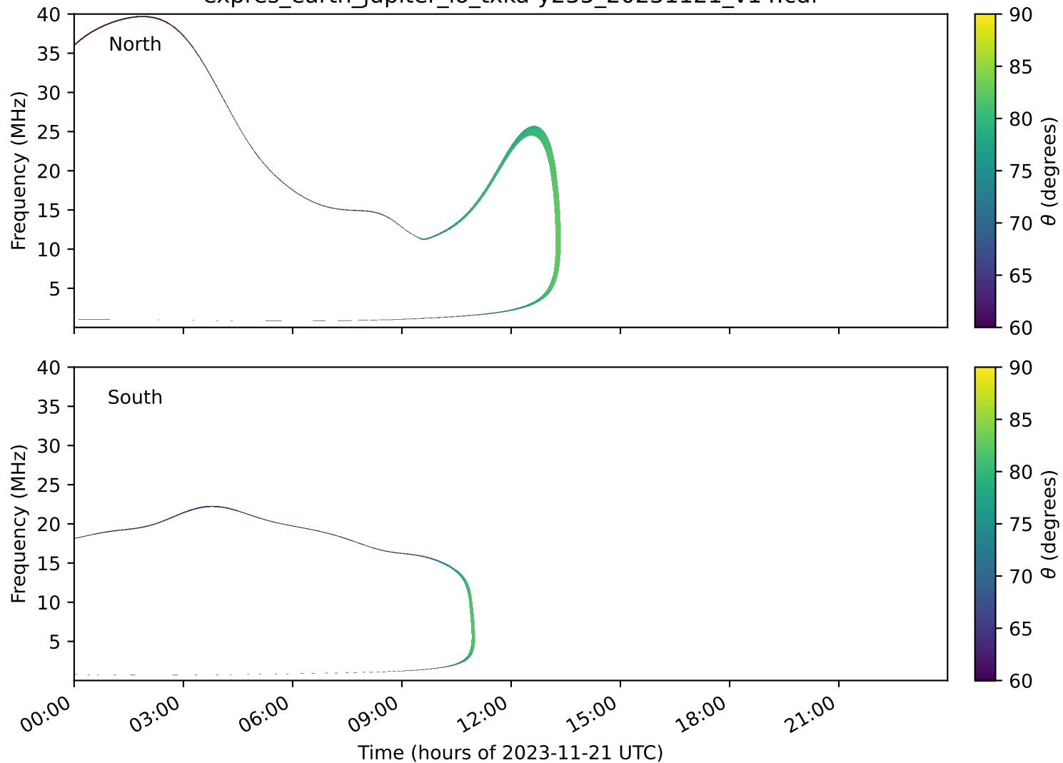
expres_earth_jupiter_io_txka-y235_20231121_v14.cdf
