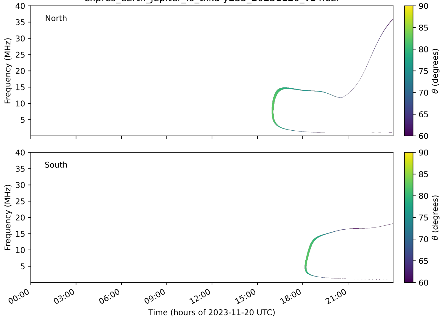
expres_earth_jupiter_io_txka-y235_20231120_v14.cdf
