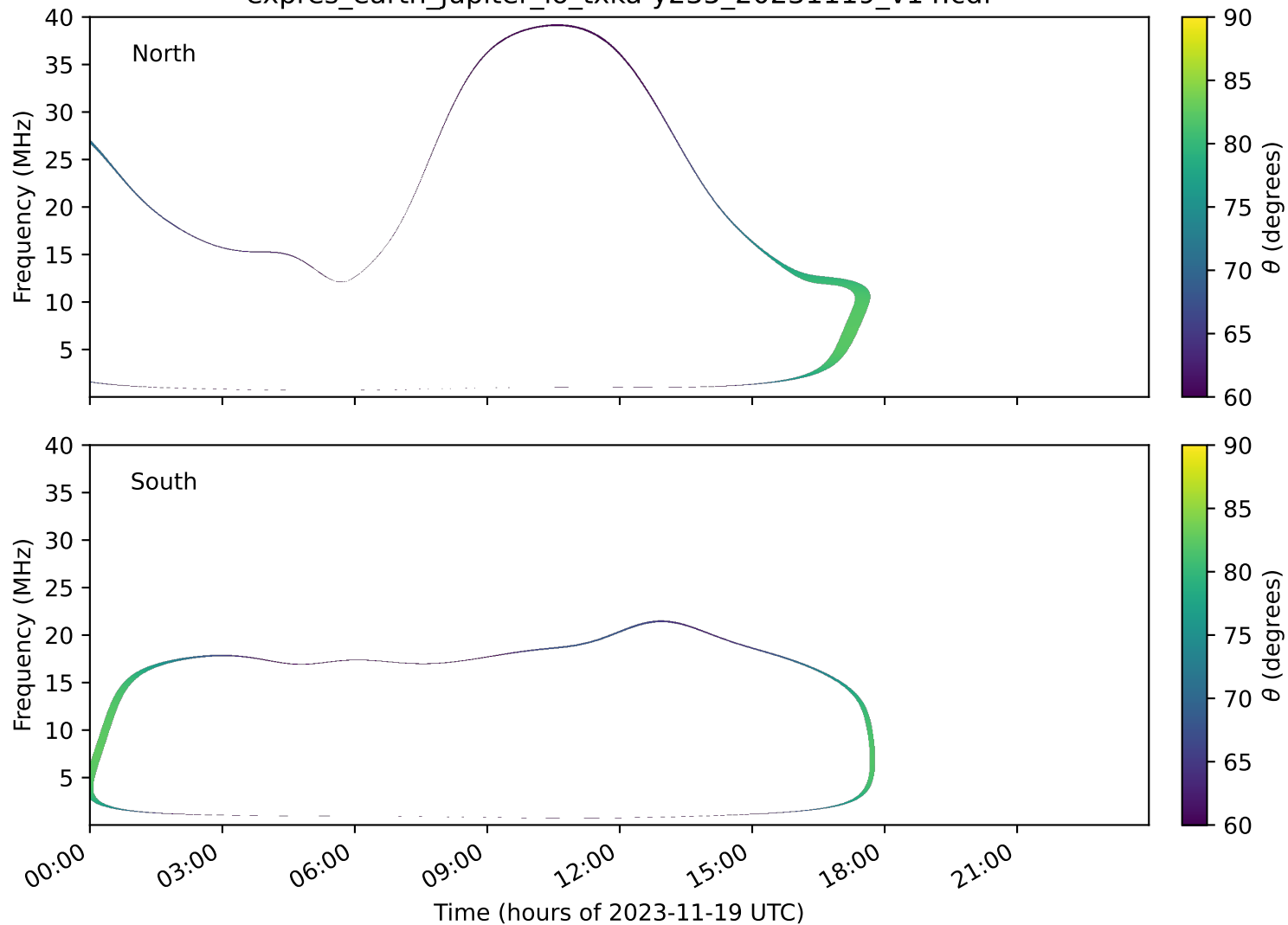
expres_earth_jupiter_io_txka-y235_20231119_v14.cdf
