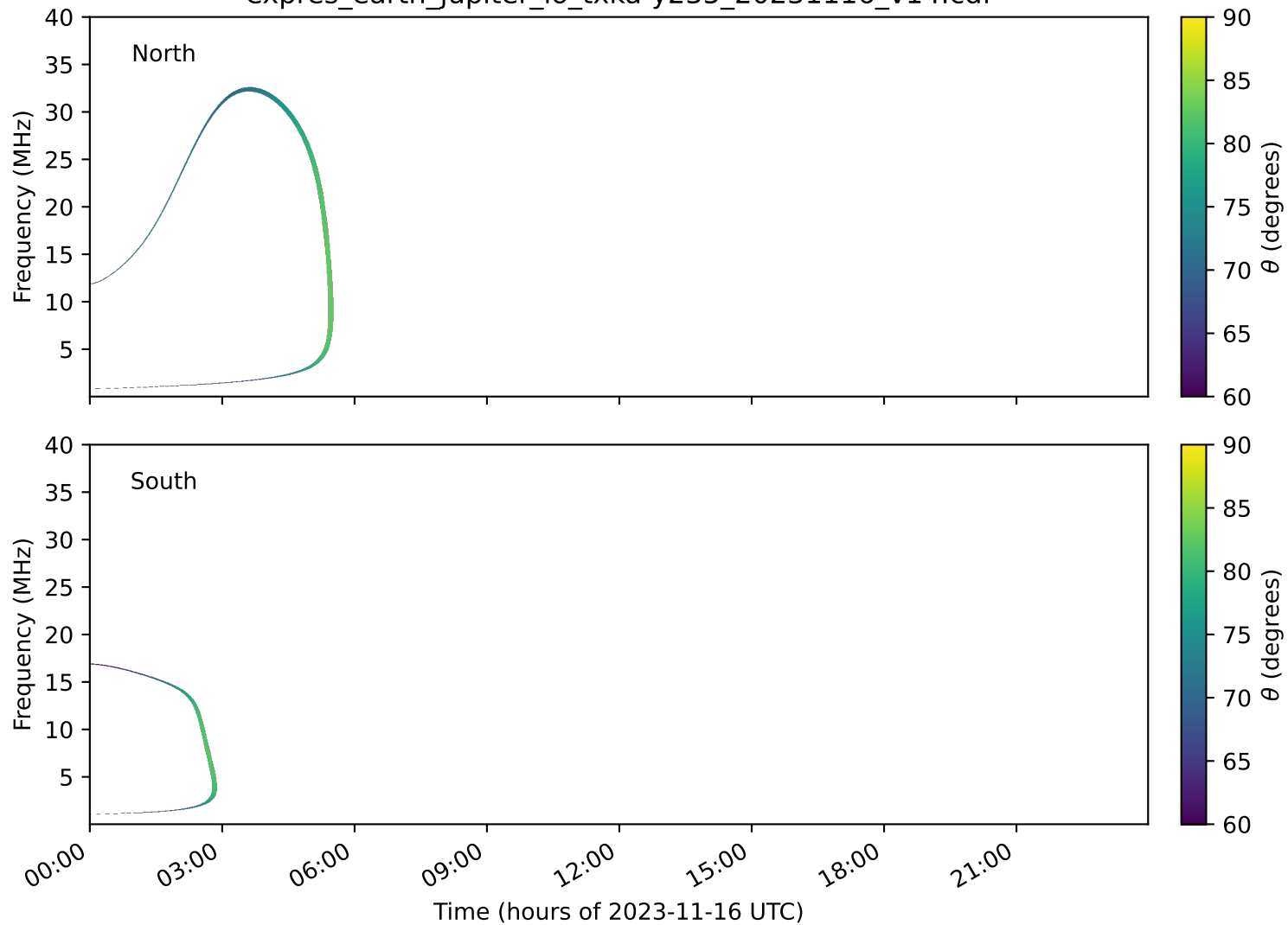
expres_earth_jupiter_io_txka-y235_20231116_v14.cdf
