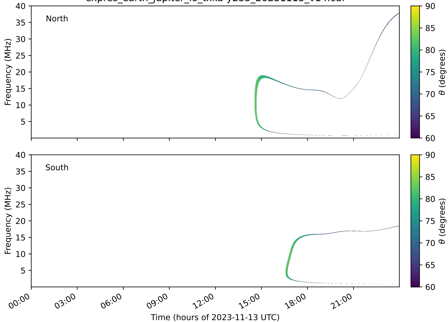
expres_earth_jupiter_io_txka-y235_20231113_v14.cdf
