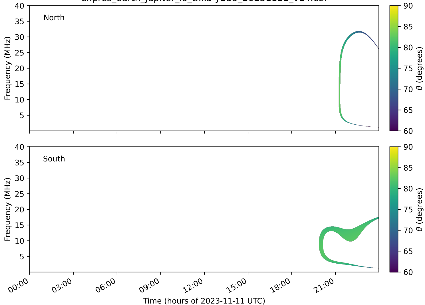
expres_earth_jupiter_io_txka-y235_20231111_v14.cdf
