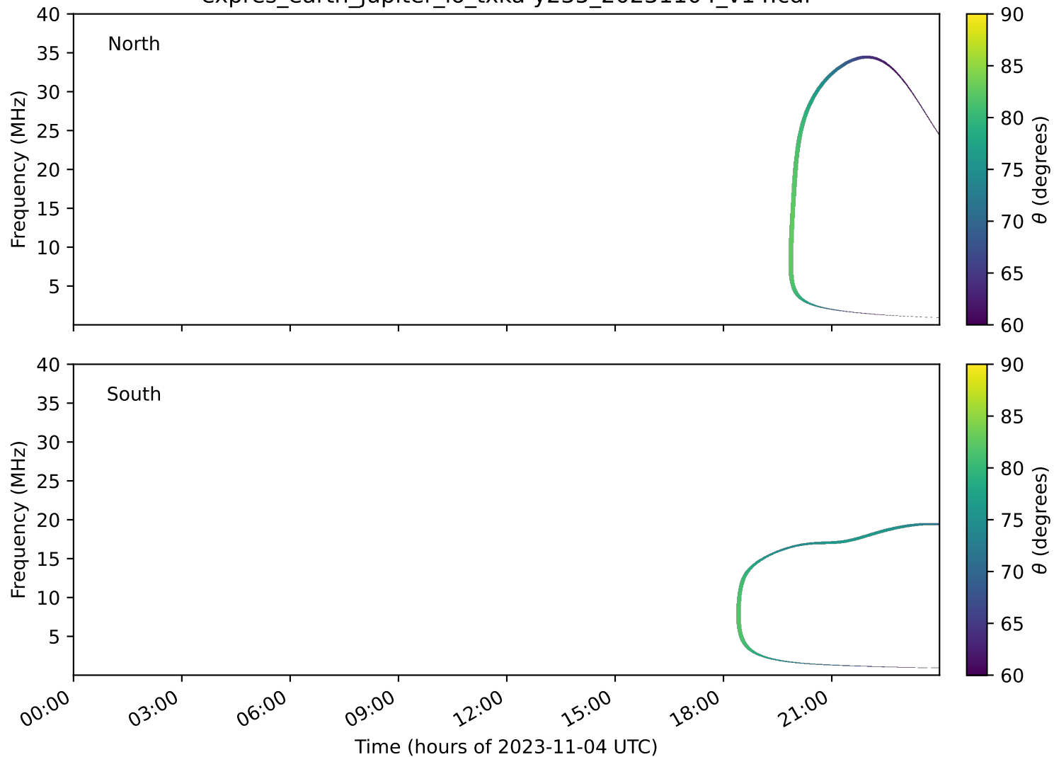
expres_earth_jupiter_io_txka-y235_20231104_v14.cdf
