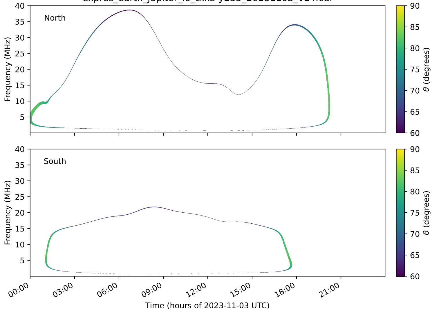
expres_earth_jupiter_io_txka-y235_20231103_v14.cdf
