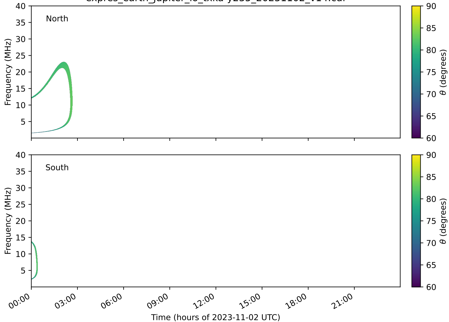
expres_earth_jupiter_io_txka-y235_20231102_v14.cdf
