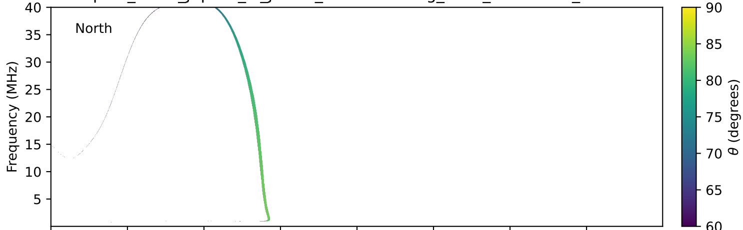
expres_earth_jupiter_io_jrm33_lossc-wid1deg_3kev_20231130_v11.cdf
