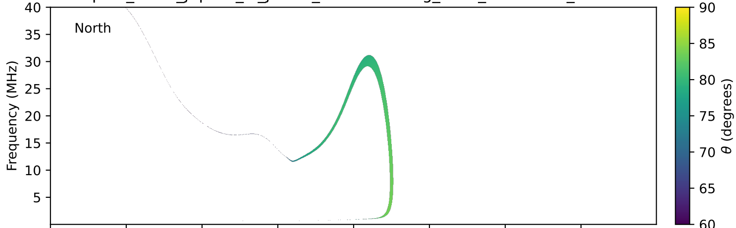
expres_earth_jupiter_io_jrm33_lossc-wid1deg_3kev_20231121_v11.cdf
