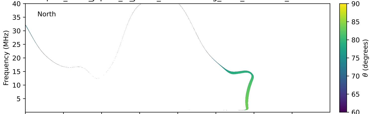
expres_earth_jupiter_io_jrm33_lossc-wid1deg_3kev_20231119_v11.cdf
