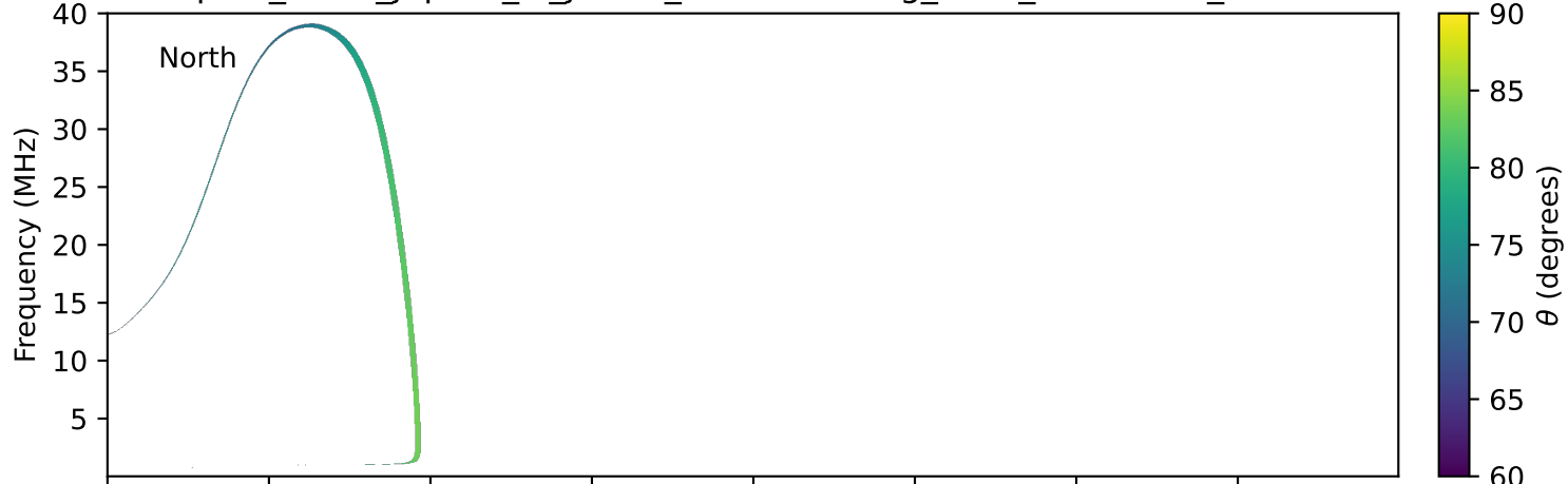
expres_earth_jupiter_io_jrm33_lossc-wid1deg_3kev_20231116_v11.cdf
