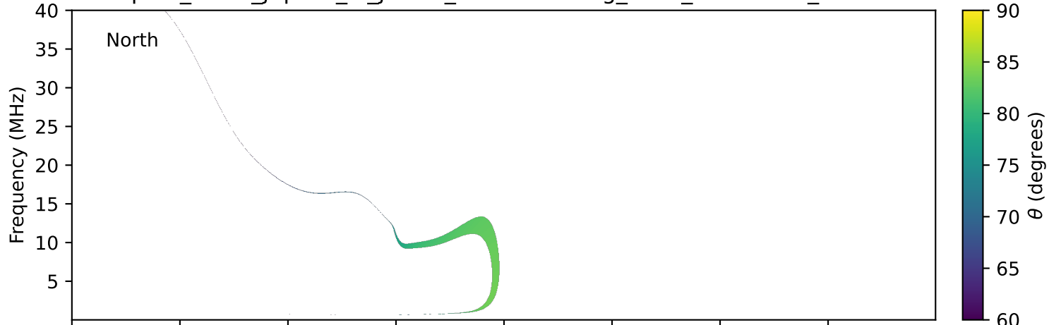
expres_earth_jupiter_io_jrm33_lossc-wid1deg_3kev_20231114_v11.cdf
