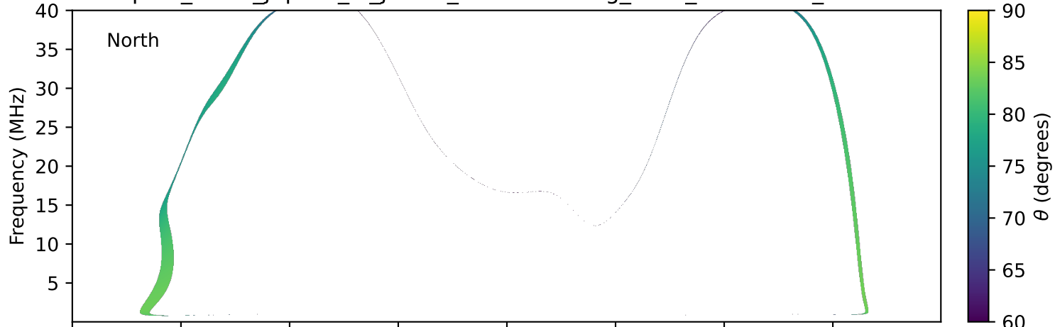
expres_earth_jupiter_io_jrm33_lossc-wid1deg_3kev_20231110_v11.cdf
