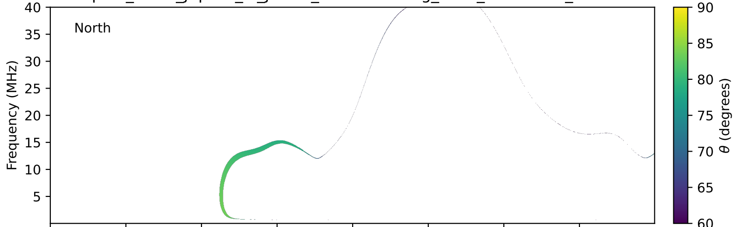
expres_earth_jupiter_io_jrm33_lossc-wid1deg_3kev_20231108_v11.cdf
