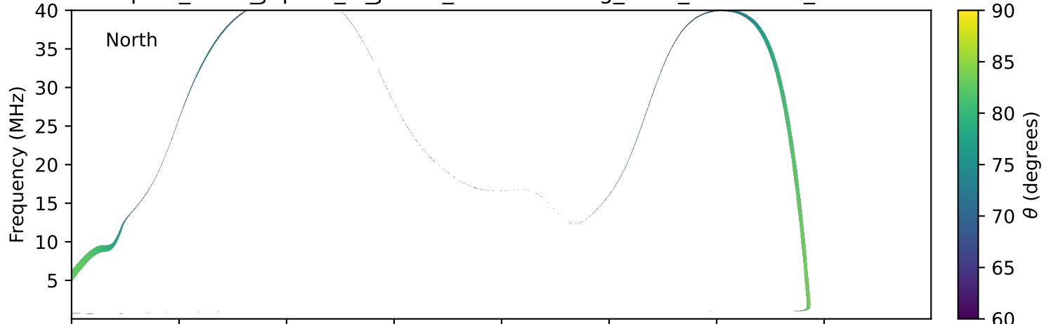
expres_earth_jupiter_io_jrm33_lossc-wid1deg_3kev_20231103_v11.cdf
