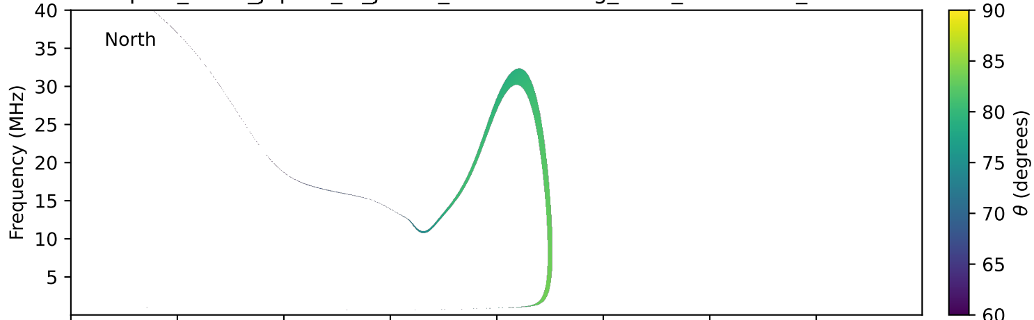
expres_earth_jupiter_io_jrm09_lossc-wid1deg_3kev_20231121_v11.cdf
