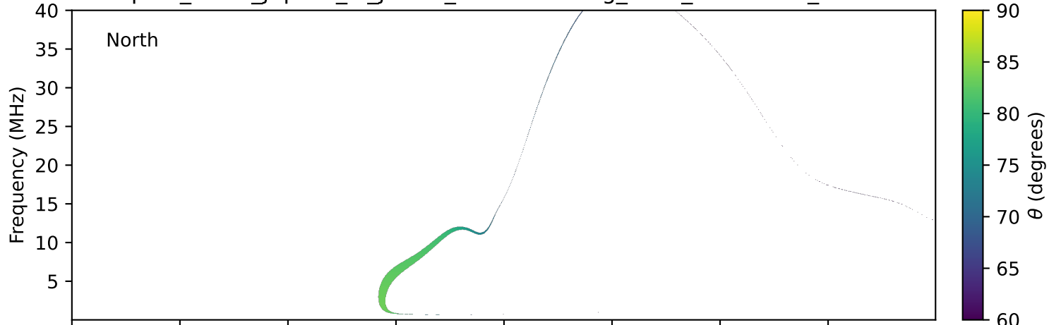
expres_earth_jupiter_io_jrm09_lossc-wid1deg_3kev_20231115_v11.cdf
