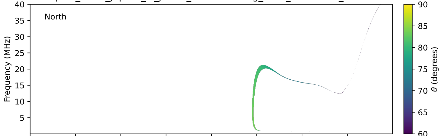
expres_earth_jupiter_io_jrm09_lossc-wid1deg_3kev_20231113_v11.cdf
