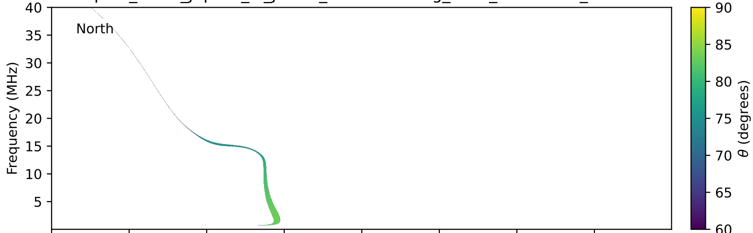
expres_earth_jupiter_io_jrm09_lossc-wid1deg_3kev_20231107_v11.cdf
