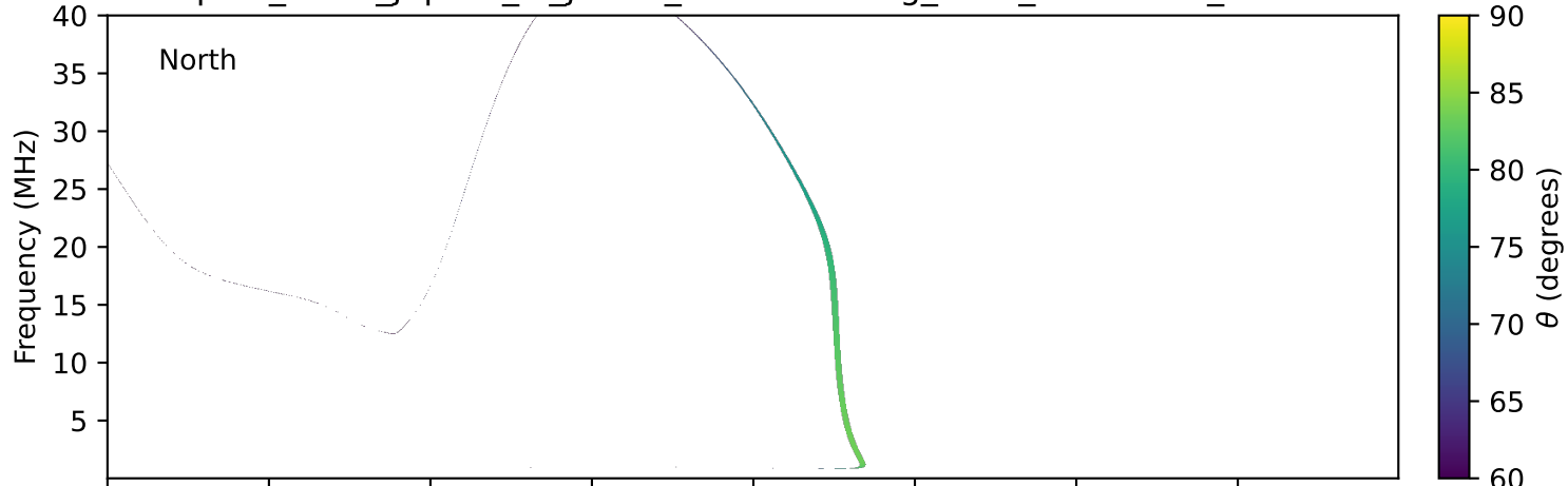
expres_earth_jupiter_io_jrm09_lossc-wid1deg_3kev_20231105_v11.cdf
