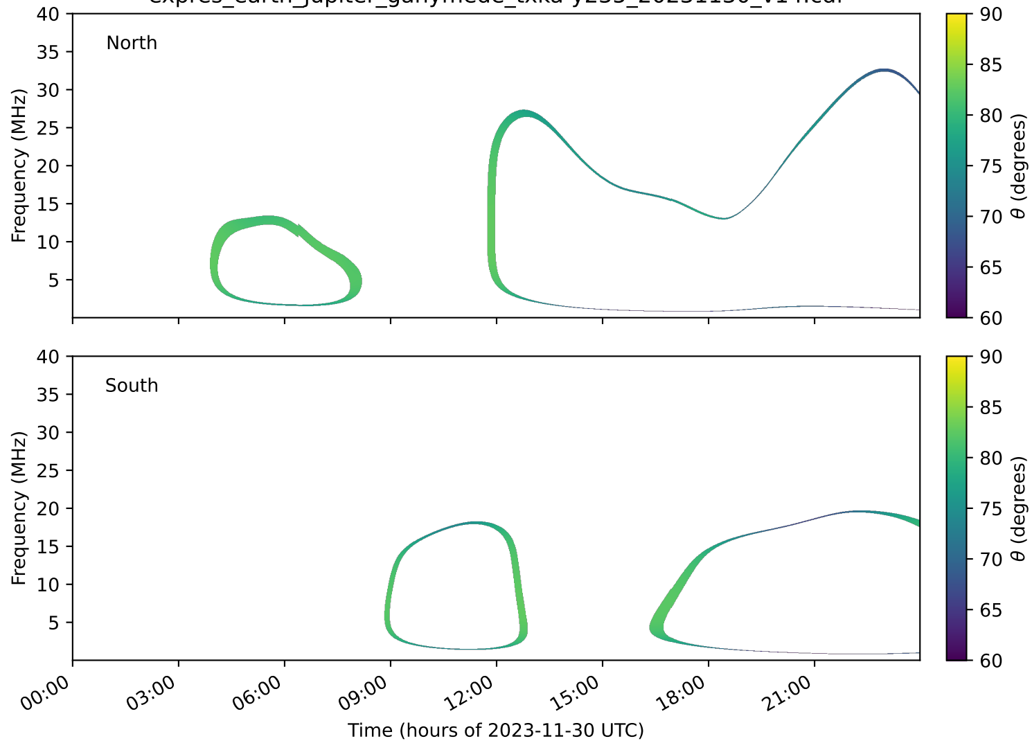
expres_earth_jupiter_ganymede_txka-y235_20231130_v14.cdf
