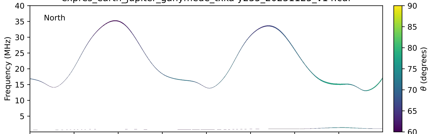
expres_earth_jupiter_ganymede_txka-y235_20231125_v14.cdf
