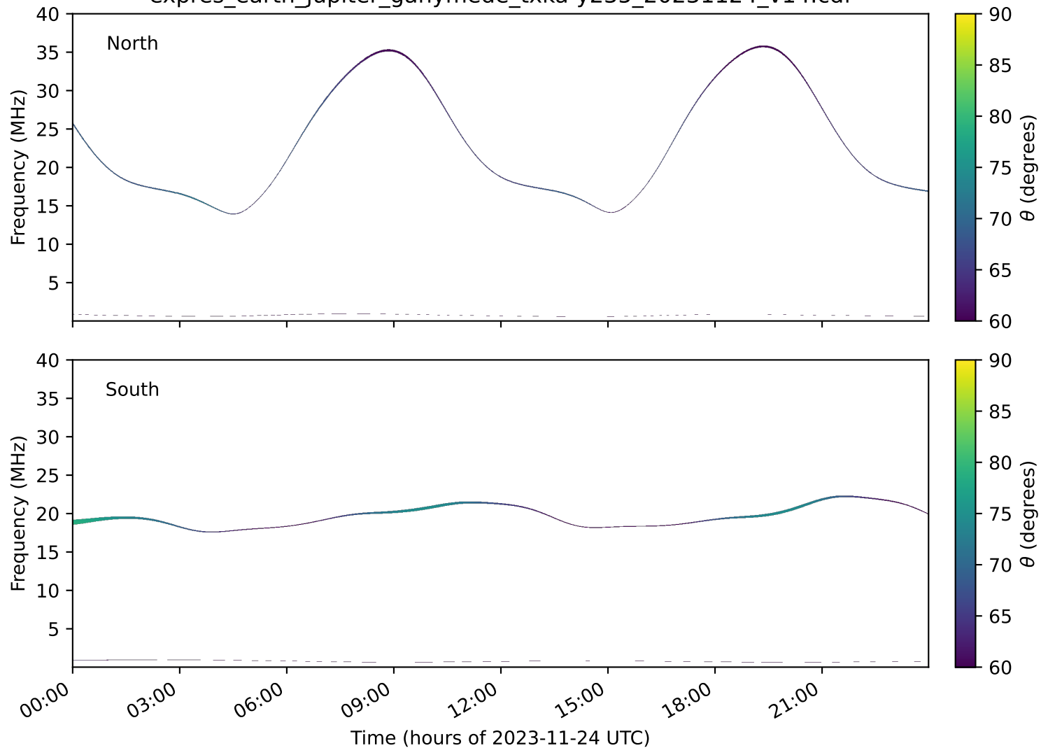
expres_earth_jupiter_ganymede_txka-y235_20231124_v14.cdf
