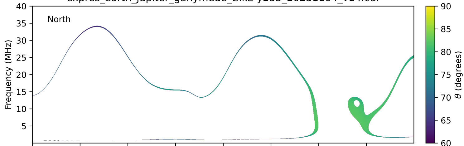
expres_earth_jupiter_ganymede_txka-y235_20231104_v14.cdf
