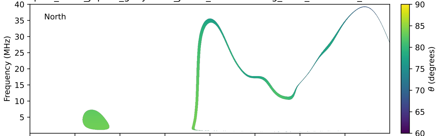
expres_earth_jupiter_ganymede_jrm33_lossc-wid1deg_3kev_20231123_v11.cdf
