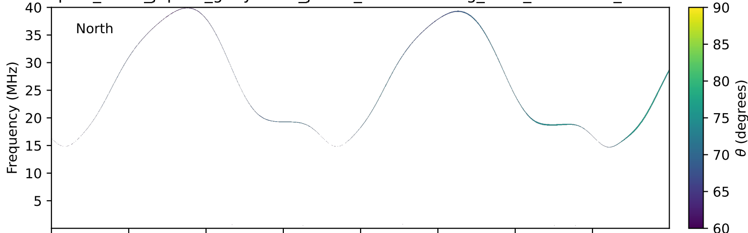
expres_earth_jupiter_ganymede_jrm33_lossc-wid1deg_3kev_20231118_v11.cdf
