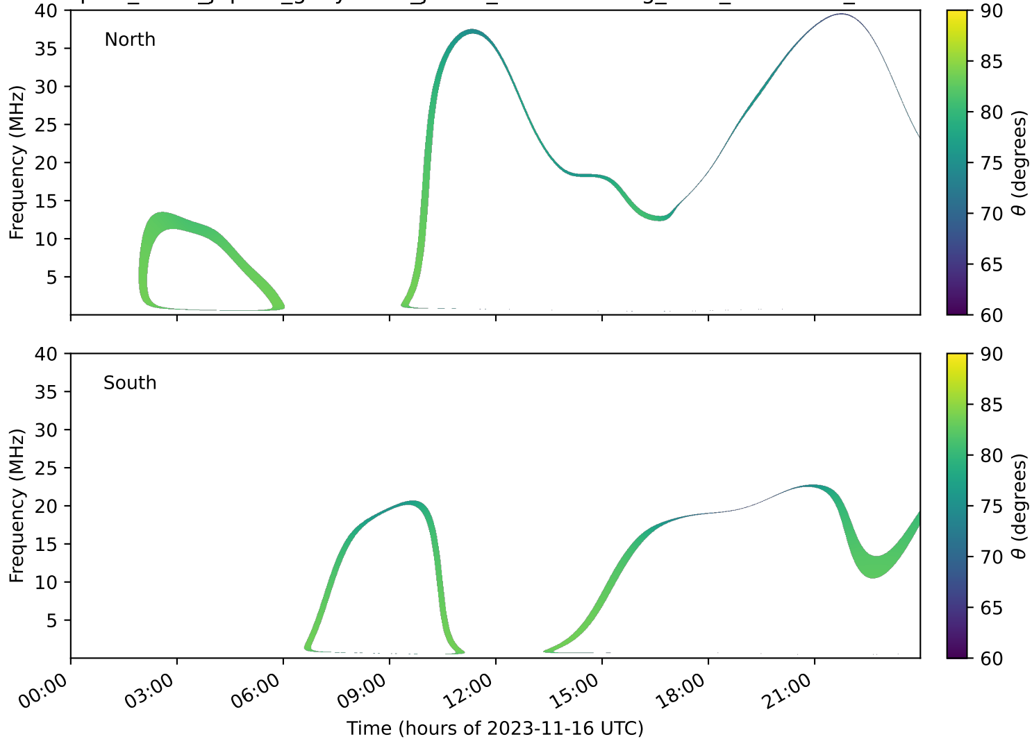
expres_earth_jupiter_ganymede_jrm33_lossc-wid1deg_3kev_20231116_v11.cdf
