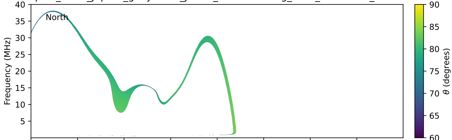
expres_earth_jupiter_ganymede_jrm09_lossc-wid1deg_3kev_20231119_v11.cdf
